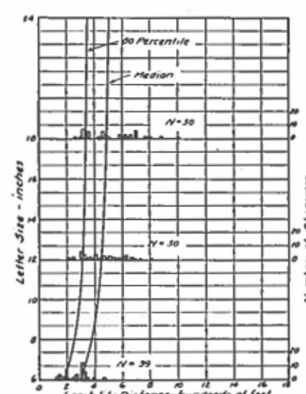
Figure 6. Night Legibility, Headlights, Black on White, Series D Letters, Reflectorized. Lighted Field, 3 Foot Lamberts. Scattered Street Lights.
