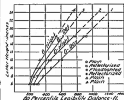
Figure 13. Practical Legibility Values Corresponding to 20/20 Vision, 80 Percentile Figures.
