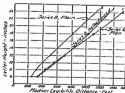
Figure 9. Effect of Width and Reflectorization, Daylight Median Values. Series D, Wider Letters. Series B, Narrower Letters.
