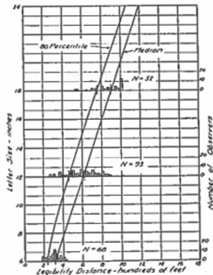
Figure 5. Night Legibility, Headlights, Black on White, Series D, Reflectorized. Dark Field, Scattered Street Lights.
