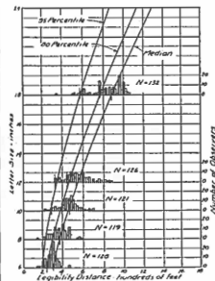
Figure 4. Night Legibility, Floodlights, Black on White, Series D Letters, Unreflectorized. Illumination 5-15 Foot Candles, Average Brightness 3 Foot Lamberts.
