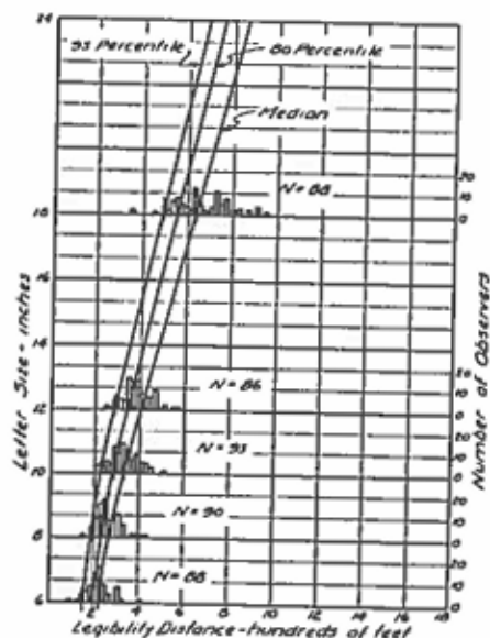
Figure 8. Night Legibility, Floodlights, Black on White, Series B Letters. Illumination 5-15 Foot Candles, Average Brightness 3 Foot Lamberts.
