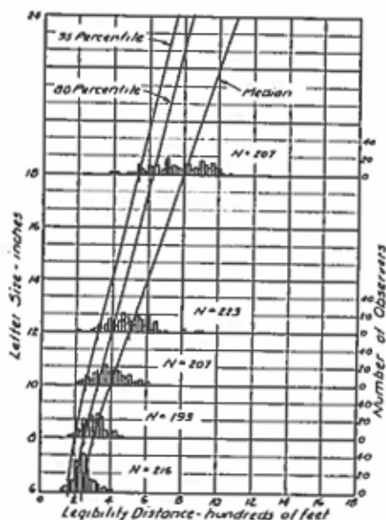
Figure 7. Daylight Legibility, Black on White, Series D Letters, Unreflectorized
