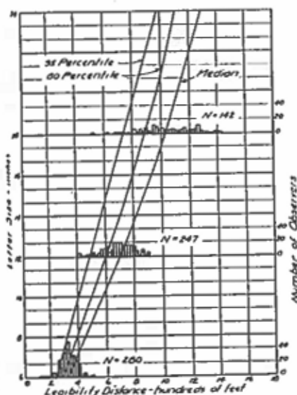
Figure 3. Daylight Legibility, Black on White, Series D Letters, Reflectorized
