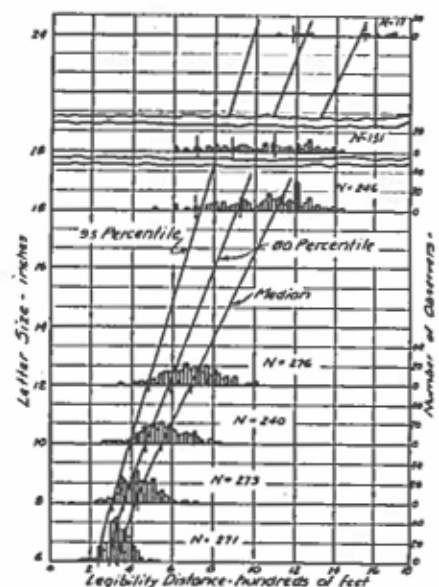
Figure 2. Daylight Legibility, Black on White, Series D Letters, Unreflectorized
