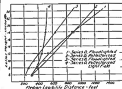
Figure 10. Effect of Width and Reflectorization at Night. Median Values
