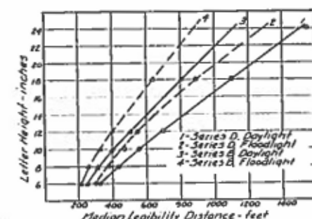
Figure 11. Comparison of Night and Day Legibility. Median Values
