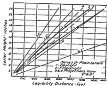
Figure 14. Error from Projection. Dotted Lines Indicate Projected Values from Small Letters Alone on the Assumption of a Linear Relationship.
