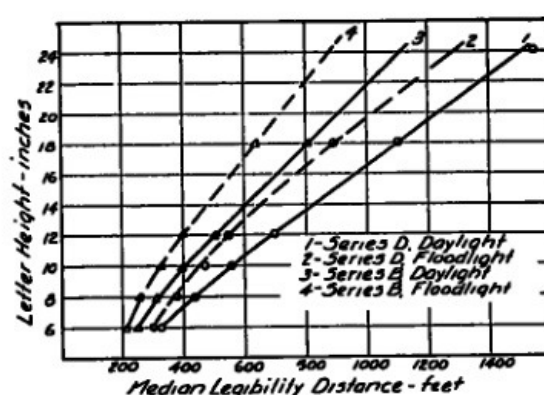
Figure 11. Comparison of Night and Day Legibility. Median Values
