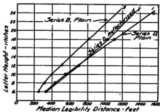
Figure 9. Effect of Width and Reflectorization, Daylight Median Values. Series D, Wider Letters. Series B, Narrower Letters.
