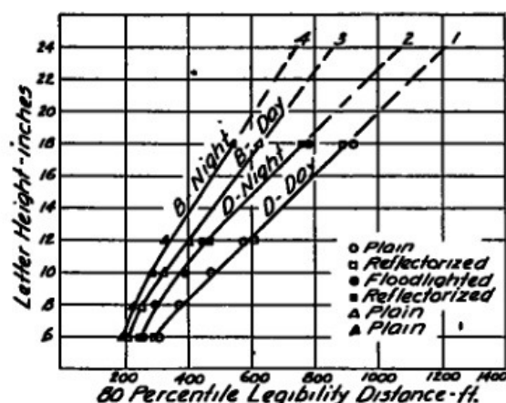
Figure 13. Practical Legibility Values Corresponding to 20/20 Vision, 80 Percentile Figures.
