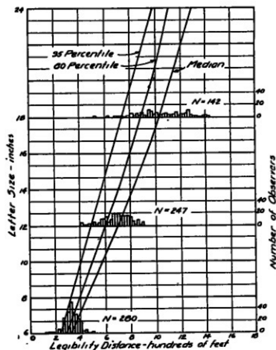
Figure 3. Daylight Legibility, Black on White, Series D Letters, Reflectorized
