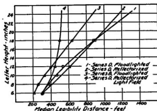
Figure 10. Effect of Width and Reflectorization at Night. Median Values
